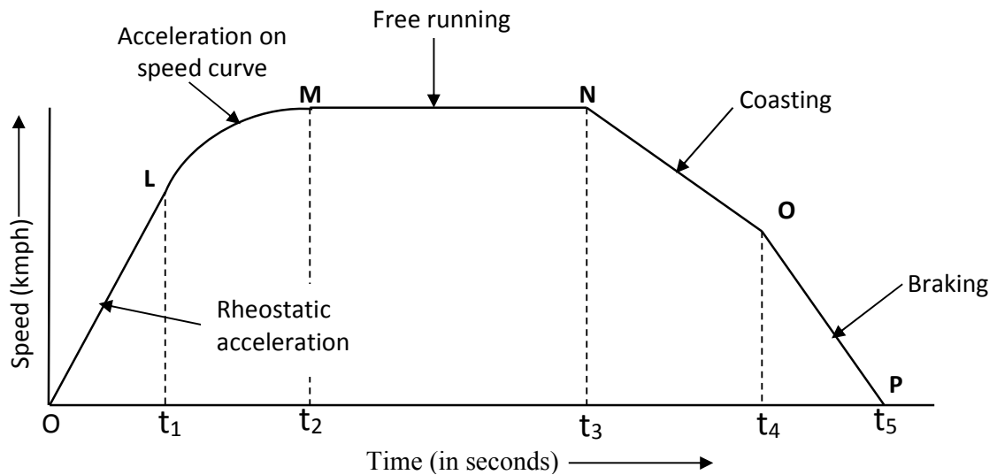
Fig. 1 Actual Speed Time Curve of Train
