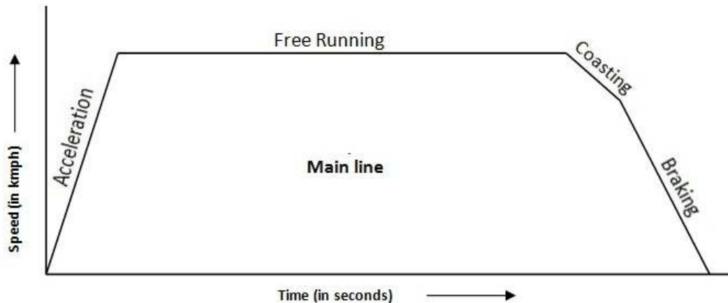
Fig.5 (b) Speed Time Curves for Main line Services
