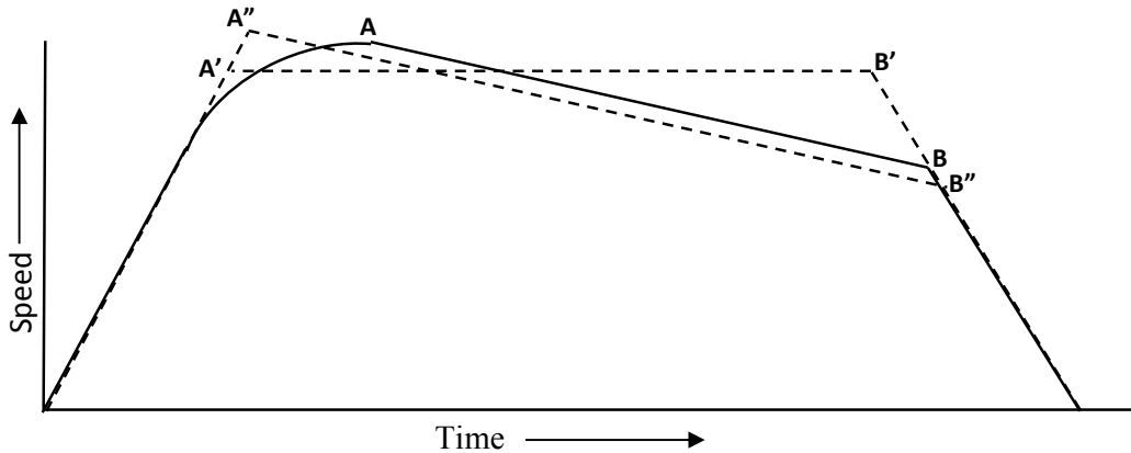
Fig.2 Simplified Speed Time Curve
