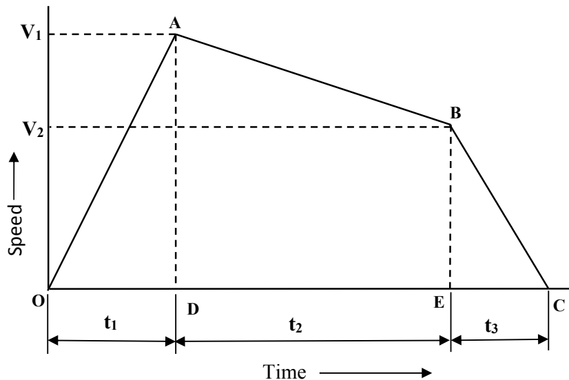
Fig.4 Simplified Quadrilateral Speed Time Curve
