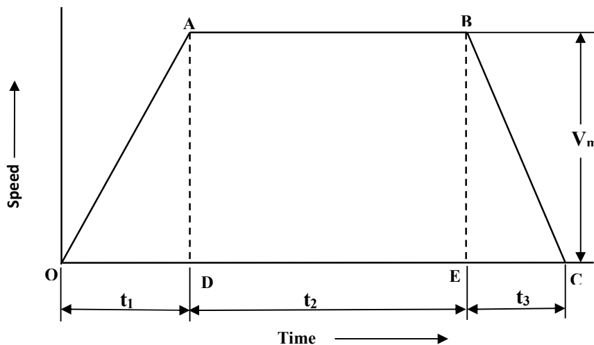
Fig.9 Trapezoidal Speed Time Curve
